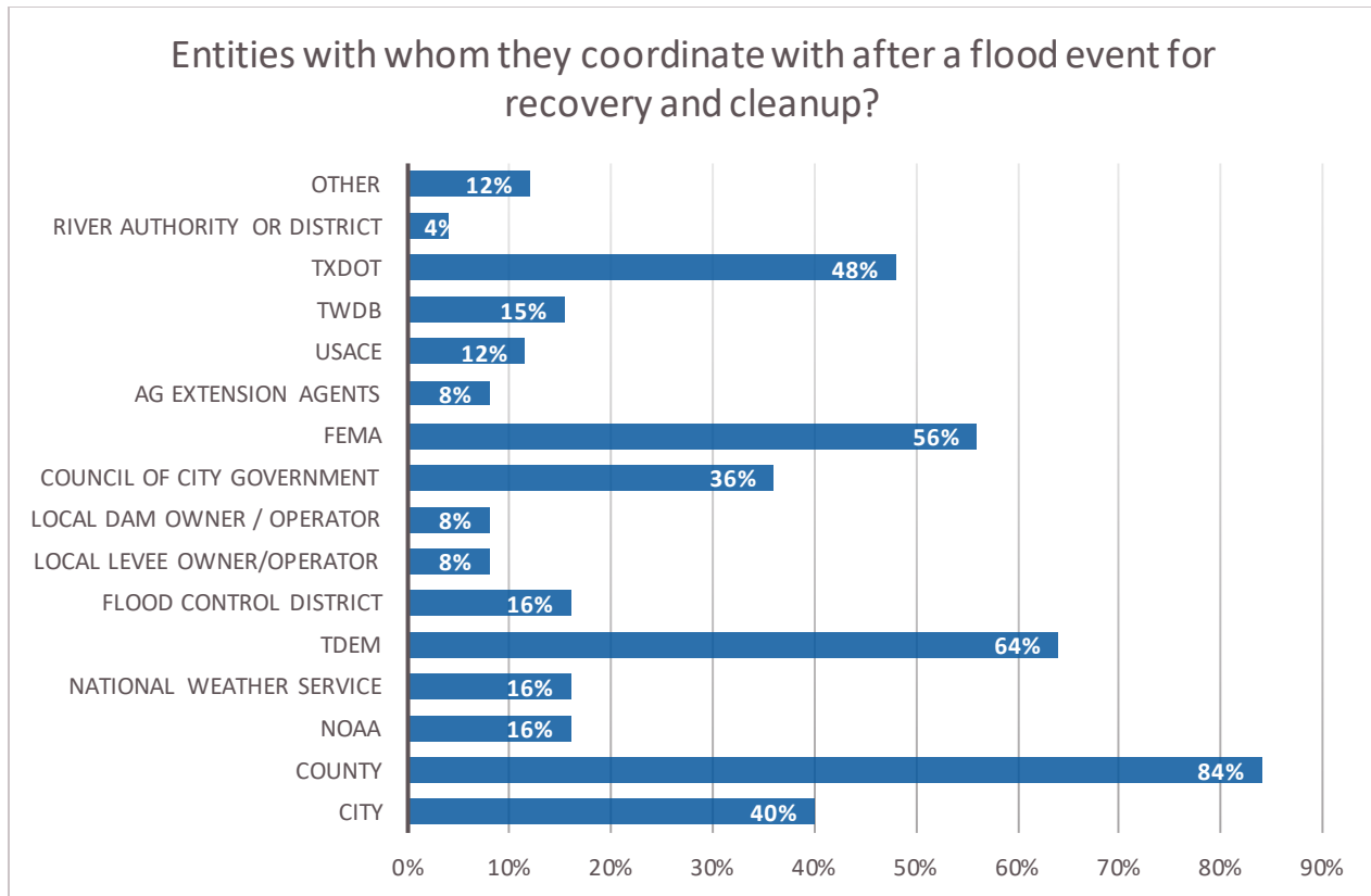
Figure 7.7 Survey question to Lower Rio Grande Planning Region’s Entities asking which entity they coordinated with after a flood event for recovery and cleanup.
